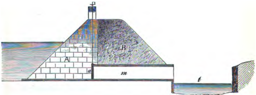
Fig. 242.—Sluice-gate of the tank A .
